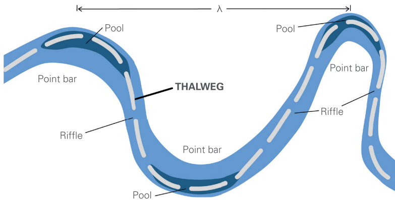
Figure 2.6 Diagram showing the locations of pools and riffles in the meander bends from Figure 2.4, and the path of the thalweg, swinging from side to side along the channel, from pool to pool on the outsides of bends. \lambda (at top) marks the meander wavelength.
